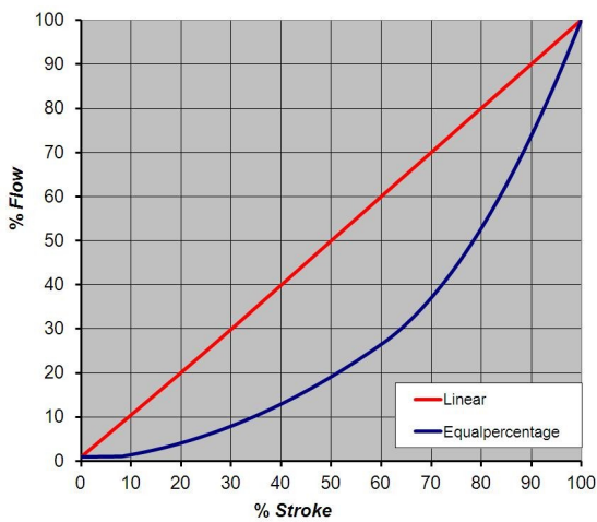
Flow rate coefficient (CV)
